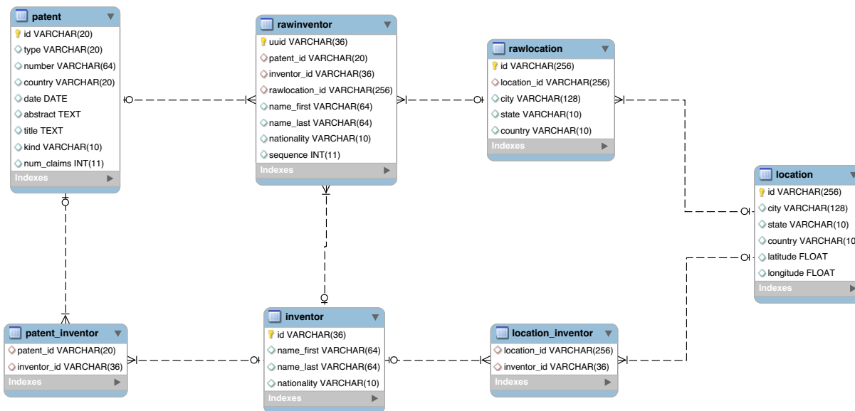
Figure 8: Inventor-related tables
