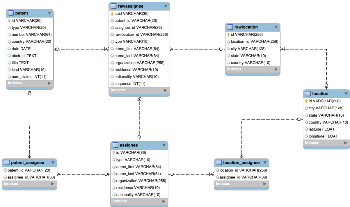
Figure 9: Assignee-related tables
